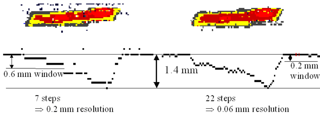
Figure 3: Effect of improving depth resolution.
