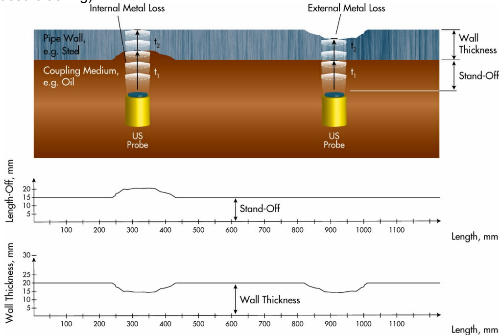
Figure 1: Ultrasound Principle Wall Thickness Measurement
