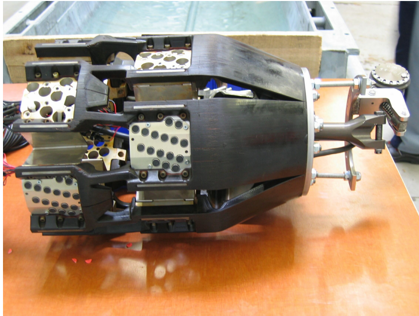
Figure 5: Sensor carrier being prepared for pitting inspection.
