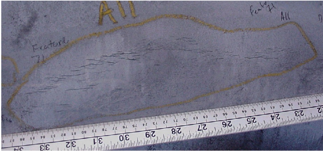
Figure 4: Typical Stress Corrosion Cracking detected with an in-line inspection tool.
